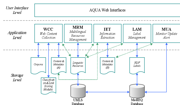
Figure 1. Architecture of the AQUA system.
